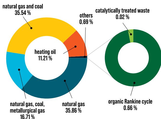
Figure 54 Share of individual CHP technologies in total CHP generation
