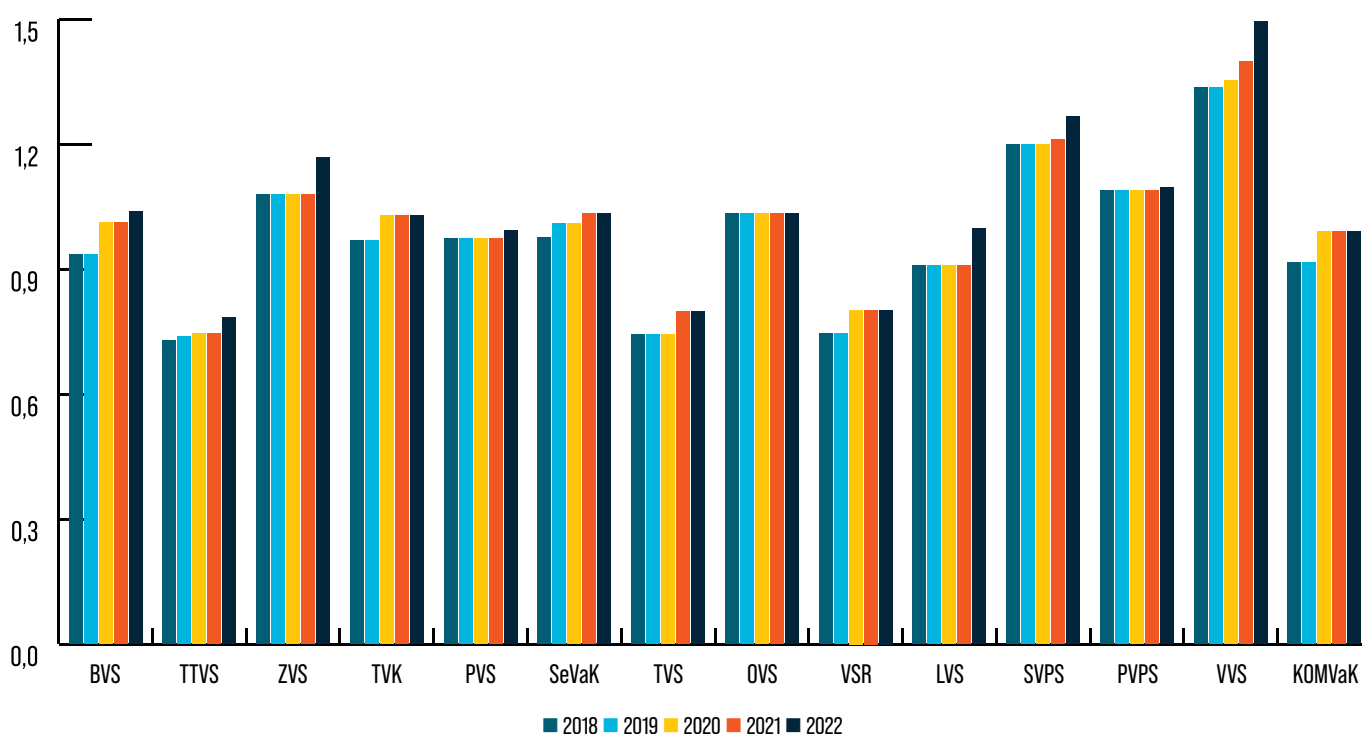
Figure 43 Evolution of prices for drinking water production and supply (€/m³)
